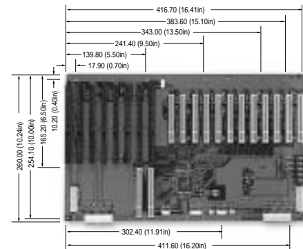
GHP-2220G 6xISA & 12xPCI & 2xPICMG CPU Slot(Single System)
