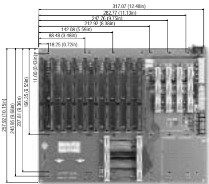
GHP-P14P4 8xISA & 4xPCI & 2xPICMG CPU Slot(Single System)
