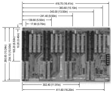
GHP-2220Q 12xPCI & 8xPICMG CPU Slot(Quad System)
