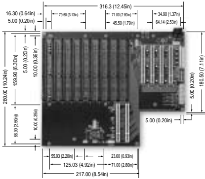
GHP-2214 8xISA & 4xPCI & 2xPICMG CPU Slot(Single System)
