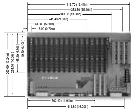
GHP-2220 13xISA & 4xPCI & 3xPICMG CPU Slot(Single System)
