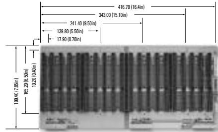
GHP-2020S 20xISA Slot(Quad System)
