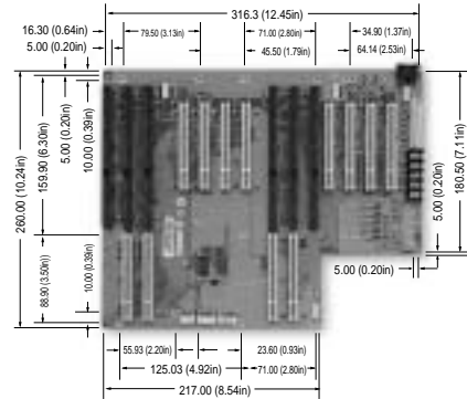
GHP-2214D 2xISA & 8xPCI & 4xPICMG CPU Slot(Dual System)
